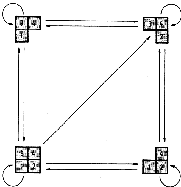
Figure 4. The directed graph of a quadtree.
