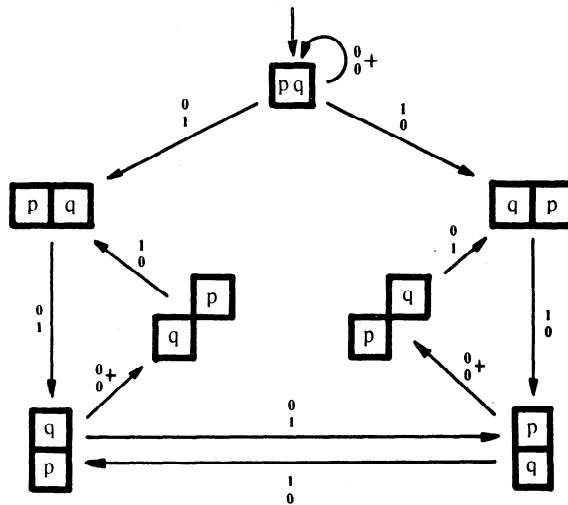
Figure 6. The directed graph for the base -1+i .
